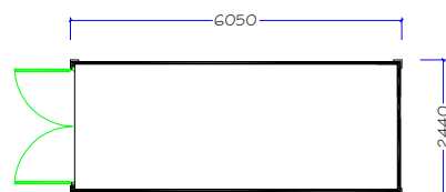
CONTAINER 20'
