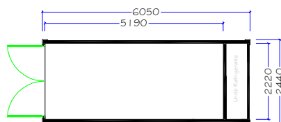
CONTAINER FRIGO 20'
