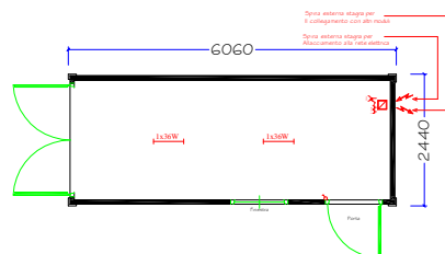
CONTAINER 20' FS.
